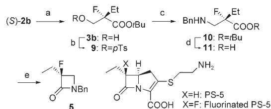
Scheme 5. Reagents and conditions: a) LiAl(O t Bu) 3 H (5.0 equiv), THF, -78^{\circ}\text{C} to RT, 1 h, 80%; b) p -TsCl (1.2 equiv), pyridine, CHCl 3 , 0^{\circ}\text{C} to RT, 12 h, 85%; c) BnNH 2 (10.0 equiv), NaHCO 3 (3.0 equiv), toluene, 80^{\circ}\text{C} , 72 h, 72%; d) TFA (5.0 equiv), CH 2 Cl 2 , 0^{\circ}\text{C} to RT, 3 h, 87%; e) 2-chloro-1-methylpyridinium iodide (1.1 equiv), triethylamine (3.0 equiv), CH 2 Cl 2 , RT, 6 h, 70%. Bn = benzyl, TFA = trifluoroacetic acid.
