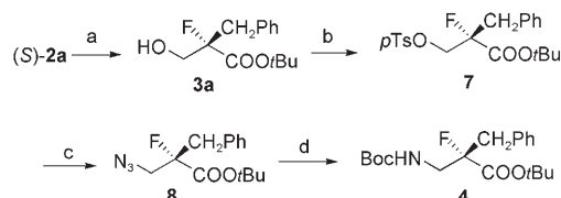
Scheme 4. Reagents and conditions: a) LiAl(O t Bu) 3 H (5.0 equiv), THF, -78^{\circ}\text{C} to RT, 1 h, 89%; b) p -TsCl (1.2 equiv), pyridine, CHCl 3 , 0^{\circ}\text{C} to RT, 12 h, 90%; c) NaN 3 (3.0 equiv), DMF, 80^{\circ}\text{C} , 24 h, 95%; d) Pd/C, H 2 , AcOEt, Boc 2 O, (1.5 equiv), RT, 2 h, 95%. Ts = 4-toluenesulfonyl, DMF = N,N -dimethylformamide, Boc = tert -butoxycarbonyl.
